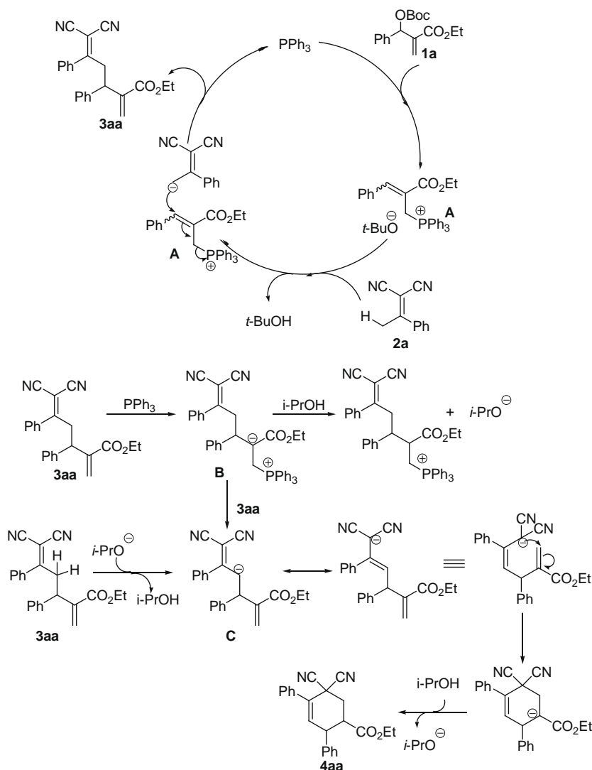
Scheme 4. Possible mechanism of the [3+3] annulation reaction.
